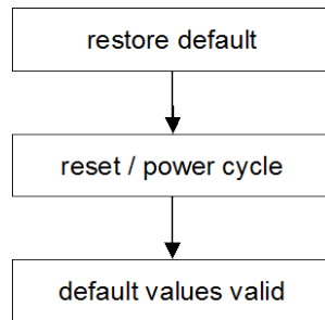
Figure 58: Restore procedure
