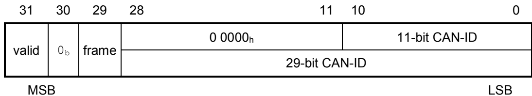
Figure 61: Structure of the EMCY Identifier
