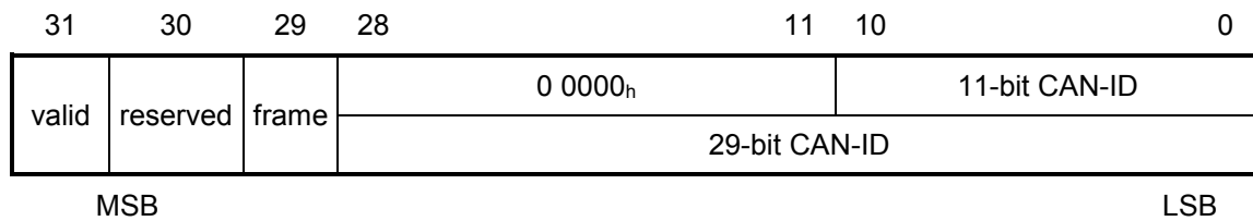
Figure 67: Structure of RPDO COB-ID
